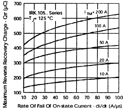
Fig. 11 - Recovery Charge Characteristics
