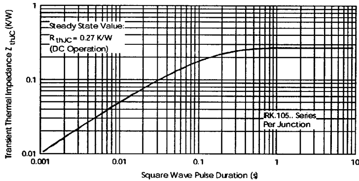
Fig. 13 - Thermal Impedance Z_{thJC} Characteristics
