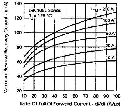
Fig. 12 - Recovery Current Characteristics
