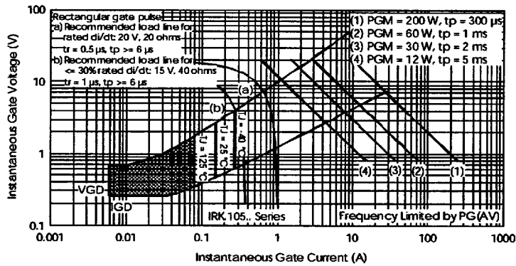
Fig. 14- Gate Characteristics
